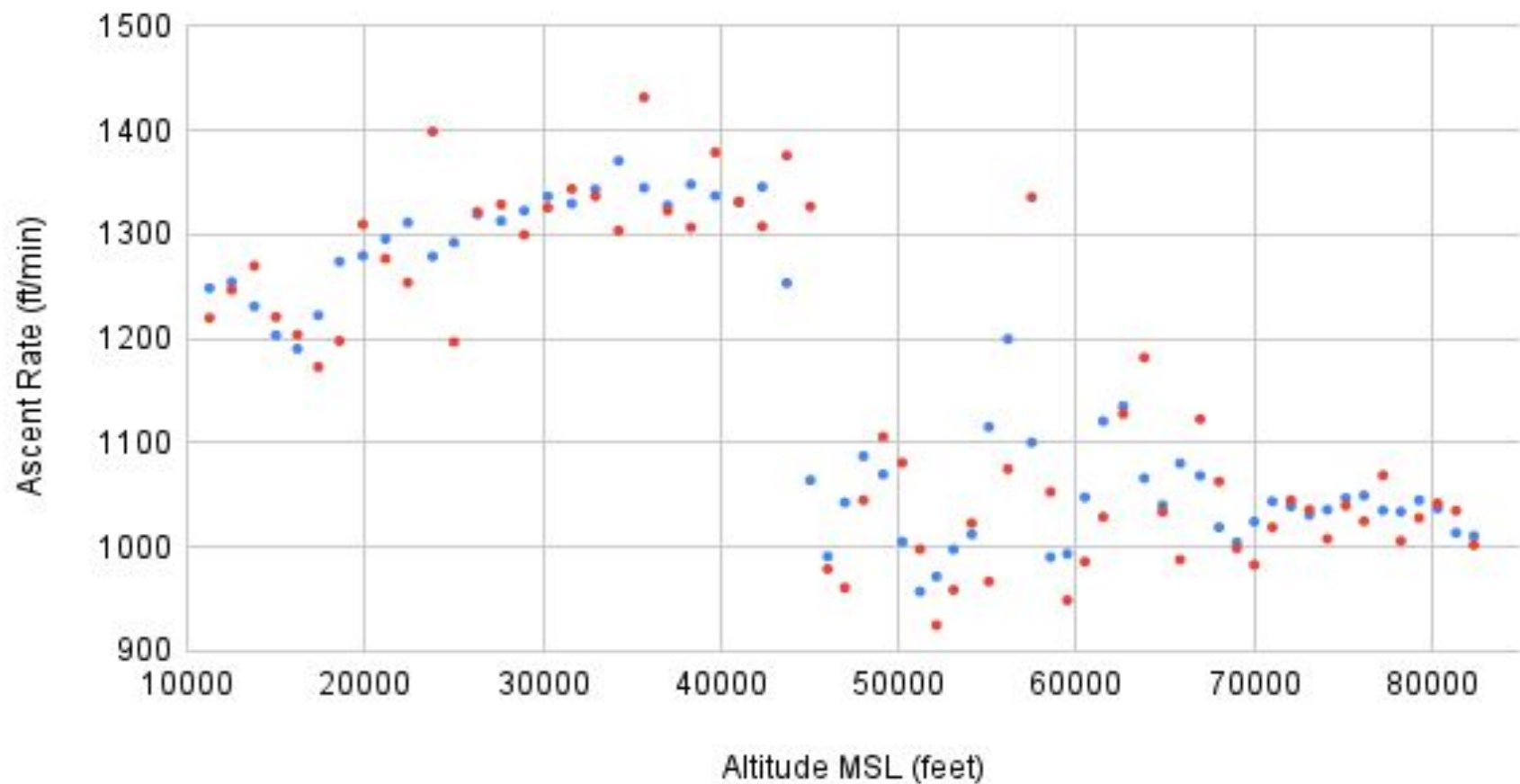
268154_3 Ascent Rate v Altitude (red=raw; blue=avg3)
