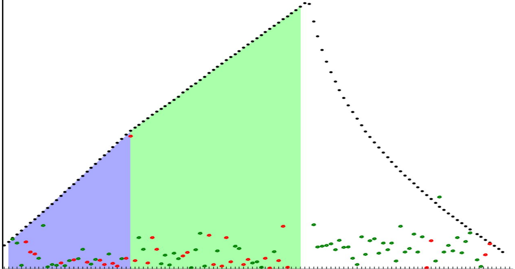
AE0SS-4 268154 Altitude (0 - 100k ft) vs. Time of Flight
